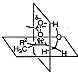
Figure 1. Stabilization of the spiro transition state through intramolecular hydrogen bonding
