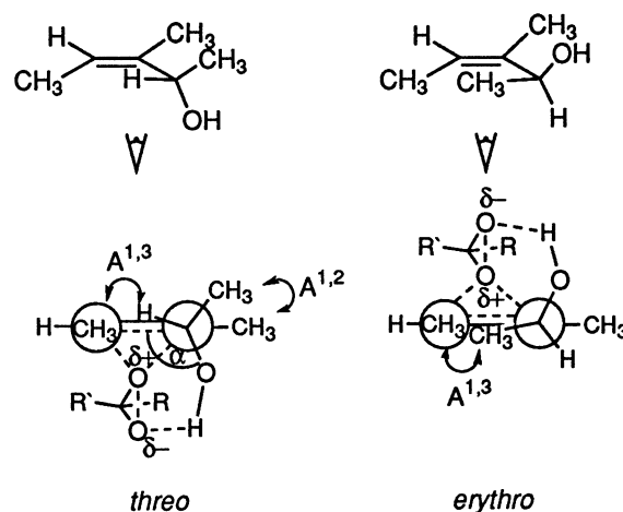
Figure 2. Diastereomeric transition states in the epoxidation of allylic alcohol 1i
